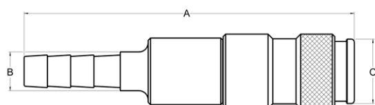
Figure 1 : Socket part
