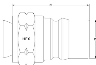
Figure 2 : Plug part
