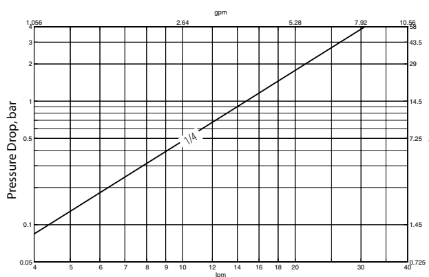
Pressure Drop Versus Flow Graph
