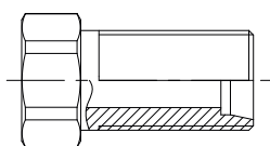
ISO 8434-1 (bulkhead version)
