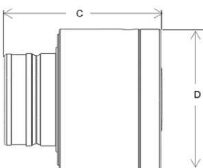
Figure 2: plug part
