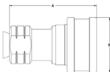
Figure 1 : Socket part
