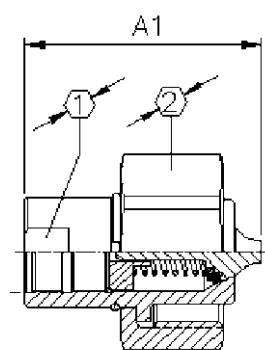
Male Half
