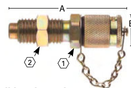
Bulkhead Couplings
