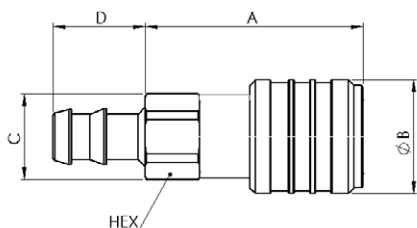
Figure 1 Push on socketless fitting
