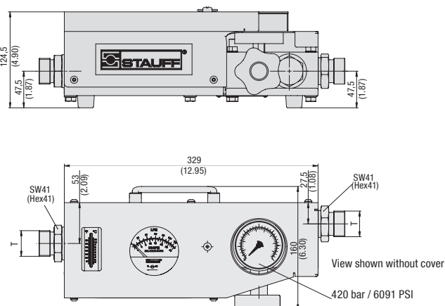
Dimensions SDMKR-750
