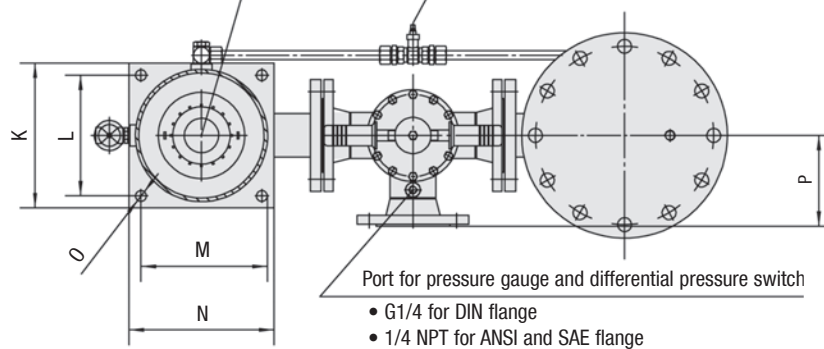
Arrangement of filter elements (see detail above)
