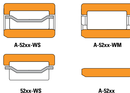
Fig. 2. 5200 metric series bearings.
