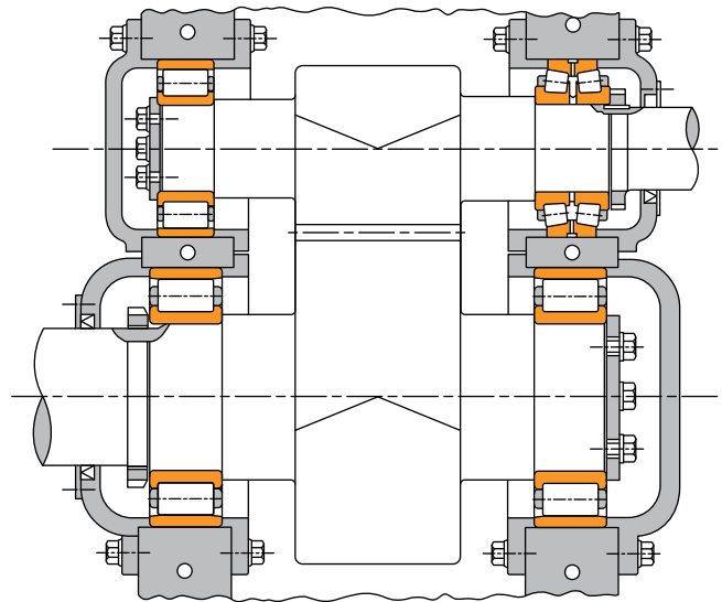
Fig. 11. Single-reduction gear reducer.
