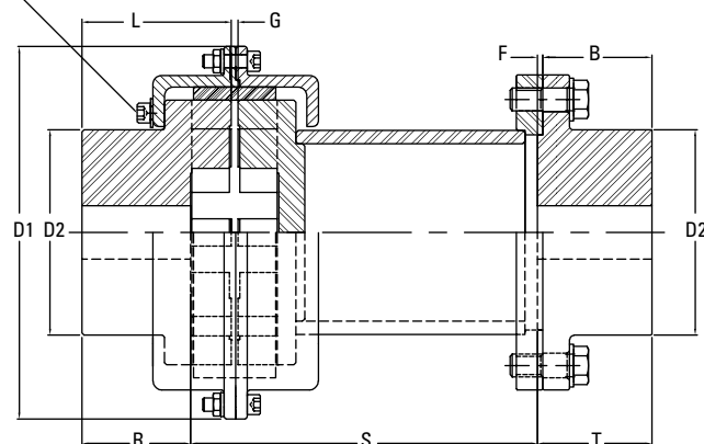
Fig. 26. Single-ended spacer coupling with high-speed split cover.
