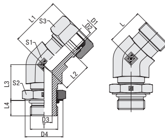
Dimensions L, L1, L2 and L3 deviating from the dimension table on the left.
