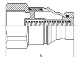
Muffe / female
