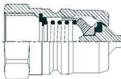
Stecker / male
