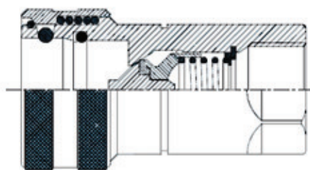
Muffe / female
