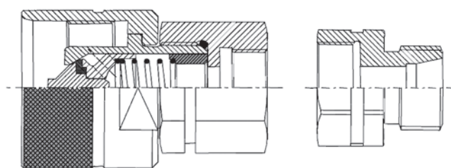
Stecker / male
