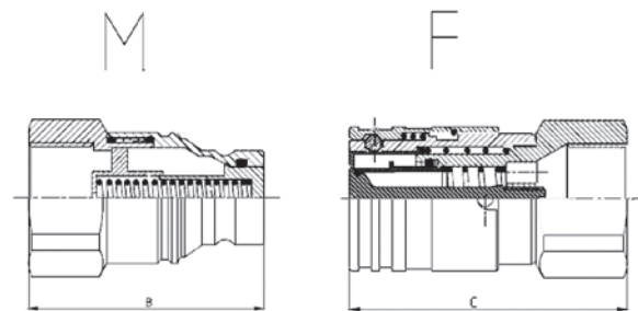
ISO 16028-Strd. 19.06
