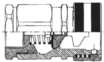
Muffe / female
