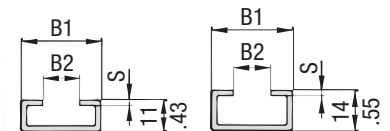
Mounting Rail TS-11 Mounting Rail TS-14
