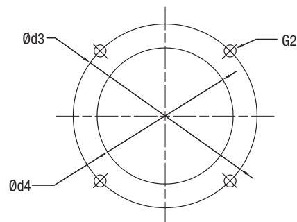
Mounting Detail
