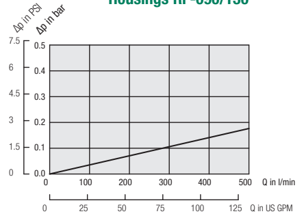
Housings RF-090/130
